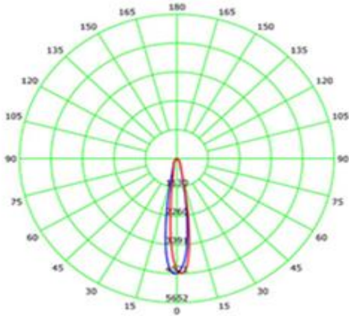
Luminous Intensity Distribution Curve(cd/klm)
